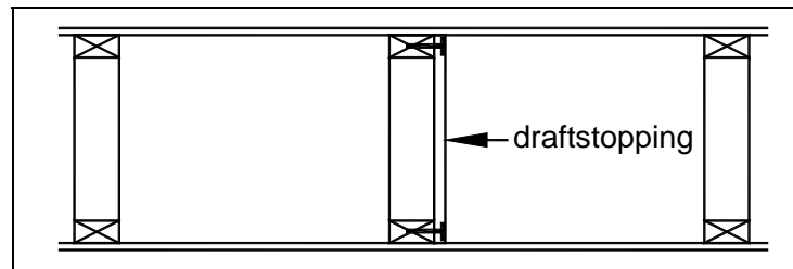
FIGURE 9: DRAFTSTOPPING AT OPEN WEB TRUSSES
